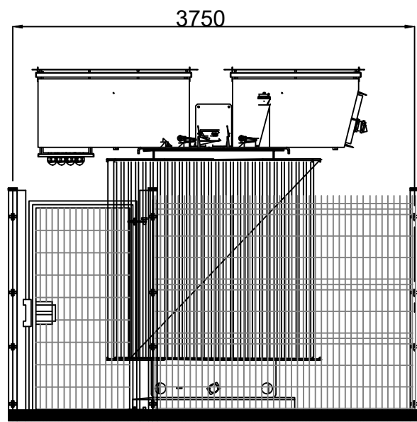
Side Elevation
