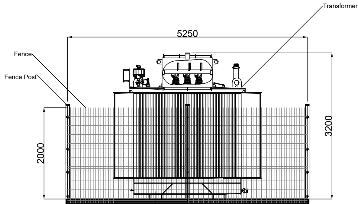
Front Elevation
